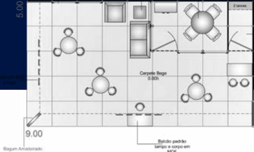
Floor plan - Shell Plus (31 to 60sqm)
